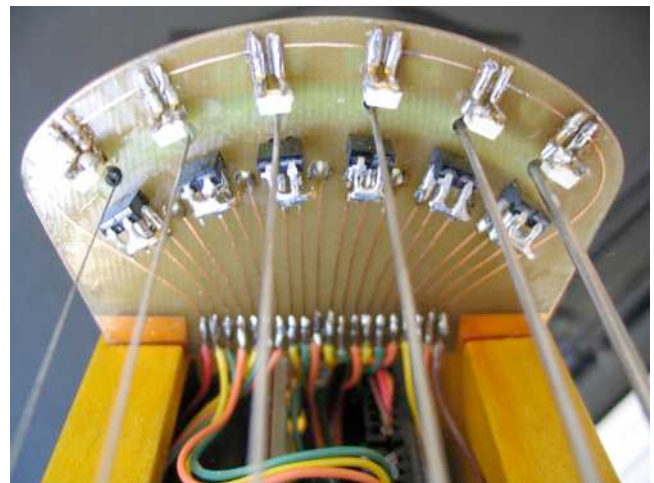
Figure 2. Overtone Violin bridge/PCB with optical pickups.
